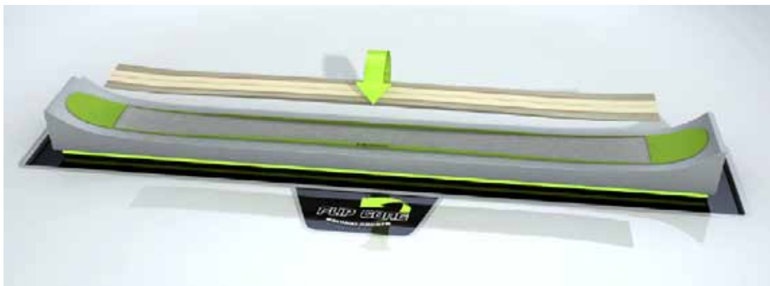
Step 1: All parts are matching exactly into the mould. The 3D woodcore is flipped upside down.
